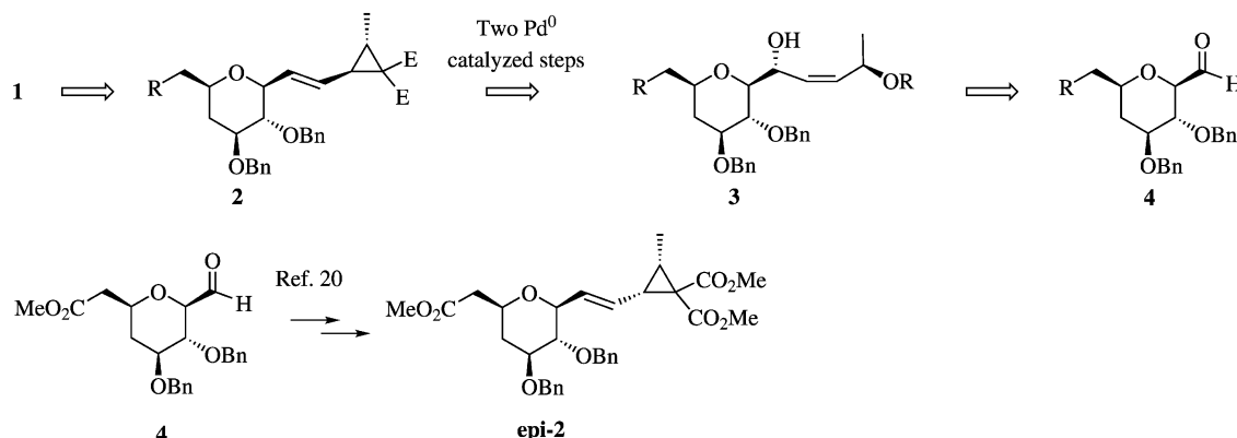
Scheme 2. Retrosynthesis of ambruticin
