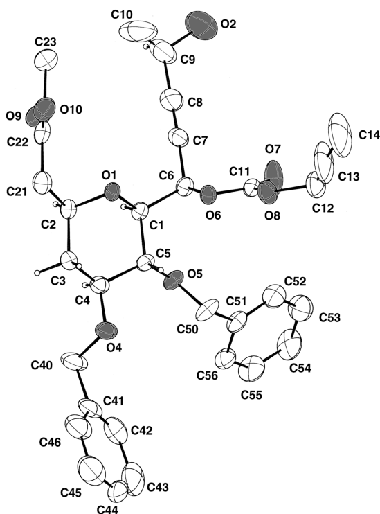
Figure 2. ORTEP drawing of the crystal structure of the alcohol 19
