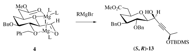
Scheme 9. Cram chelation model on aldehyde 4
