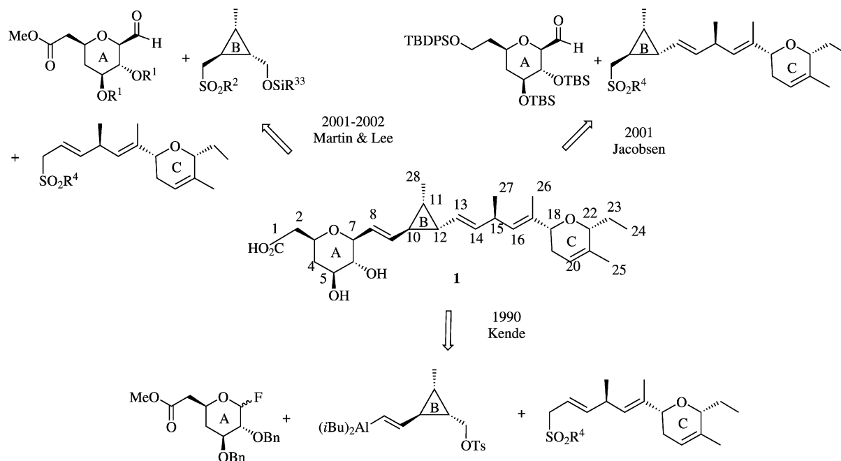
Scheme 1. Total syntheses of ambruticin
