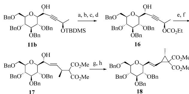
Scheme 7. Synthesis of the tetra- O -benzylated western part of ambruticin; a) ClCO 2 CH 2 CH=CH 2 , pyridine, CH 2 Cl 2 , 0 °C – room temp., 95%; b) Bu 4 NF, THF, 0 °C – room temp., 92%; c) ClCO 2 Et, pyridine, CH 2 Cl 2 , 0 °C – room temp., 92%; d) Pd(OAc) 2 (20 mol %)/TPPTS, CH 3 CN/H 2 O (6:1), Et 3 NH, room temp., 83%; e) Pd/C (10 mol %), pyridine (5 mol %), H 2 , room temp., MeOH, 70%; f) Pd(OAc) 2 (10 mol %), dppe (15 mol %), NaCH(CO 2 Me) 2 , THF, room temp., 43% (50% of SM recovered); g) 2,4-Cl 2 -C 6 H 3 COCl, pyridine, CH 2 Cl 2 , 0 °C – room temp., 71%; h) Pd(OAc) 2 (10 mol %), dppe (15 mol %), DBU, THF, room temp., 68%
