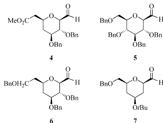
Scheme 3. Functionalized β-C-glycosyl aldehydes
