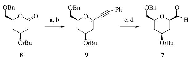
Scheme 4. Synthesis of aldehyde 7 : a) n\text{BuLi} , \text{PhC}\equiv\text{CH} , THF, -78\text{ }^\circ\text{C} – room temp., 95%; b) \text{BF}_3\cdot\text{Et}_2\text{O} , \text{Et}_3\text{SiH} , \text{CH}_3\text{CN}/\text{CH}_2\text{Cl}_2 , -40\text{ }^\circ\text{C} , 79%; c) \text{Pd/Lindlar} , \text{H}_2 (1 atm), quinoline, \text{EtOAc} , room temp., 100%; d) \text{O}_3 , \text{CH}_2\text{Cl}_2 , -78\text{ }^\circ\text{C} then \text{Me}_2\text{S} , 58%
