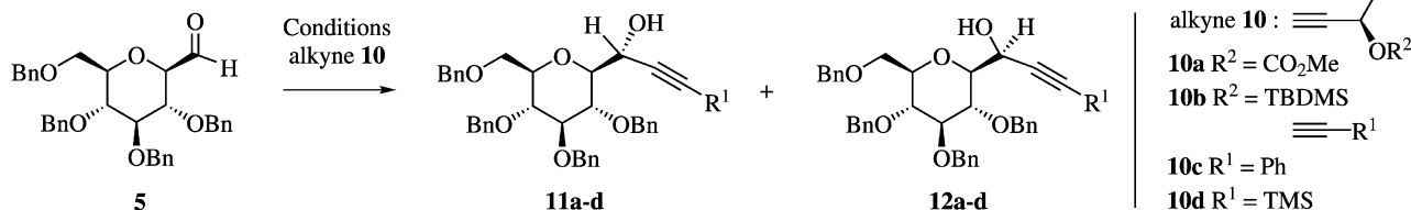
Scheme 5. Hydroxy alkylation of aldehyde 5 with various alkynyl derivatives
