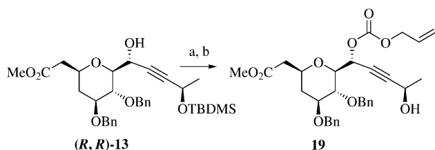
Scheme 8. Protection of alcohol (R,R)-13; a) \text{ClCO}_2\text{CH}_2\text{CH}=\text{CH}_2 , pyridine, \text{CH}_2\text{Cl}_2 , 0^\circ\text{C} – room temp., 95%; b) \text{Bu}_4\text{NF} , THF, 0^\circ – room temp., 90%
