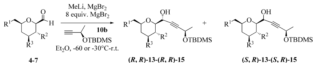
Scheme 6. Hydroxy alkylation of aldehydes 4 , 6 , and 7 with 10b
