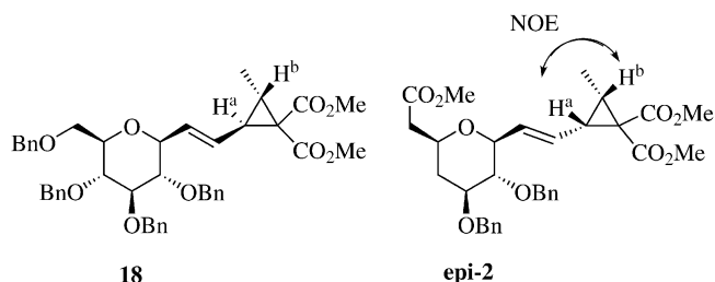
Figure 1. Comparison of cyclopropanes 18 and epi - 2
