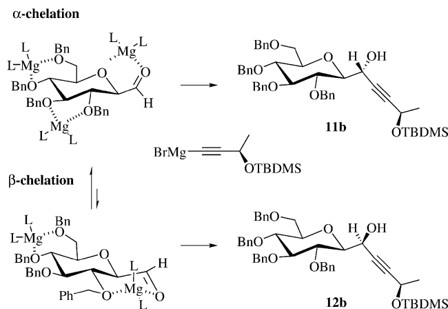
Scheme 10. Cram chelation model on aldehyde 5
