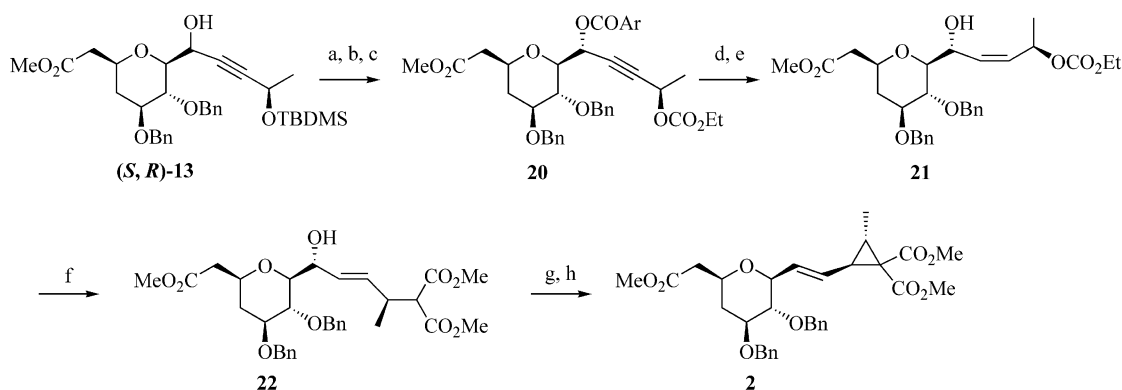
Scheme 11. Synthesis of the western part of ambruticin; a) DEAD, \text{PPh}_3 , 4- \text{NO}_2\text{-C}_6\text{H}_4\text{-CO}_2\text{H} , 90%; b) \text{Bu}_4\text{NF} , THF, 0 °C – room temp., 80%; c) \text{ClCO}_2\text{Et} , pyridine, \text{CH}_2\text{Cl}_2 , 0 °C – room temp., 92% Ar = 4- \text{NO}_2\text{-C}_6\text{H}_4 ; d) \text{K}_2\text{CO}_3 2 mol % MeOH, room temp., 70%; e) Pd/C (10 mol %), \text{H}_2 , room temp., EtOAc, 70%; f) \text{Pd}(\text{OAc})_2 (10 mol %), dppe (15 mol %), \text{NaCH}(\text{CO}_2\text{Me})_2 , THF, room temp., 80%; g) 2,4- \text{Cl}_2\text{-C}_6\text{H}_3\text{COCl} , pyridine, \text{CH}_2\text{Cl}_2 , 0 °C – room temp., 80%; h) \text{Pd}(\text{OAc})_2 (10 mol %), dppe (15 mol %), DBU, THF, room temp., 60%
